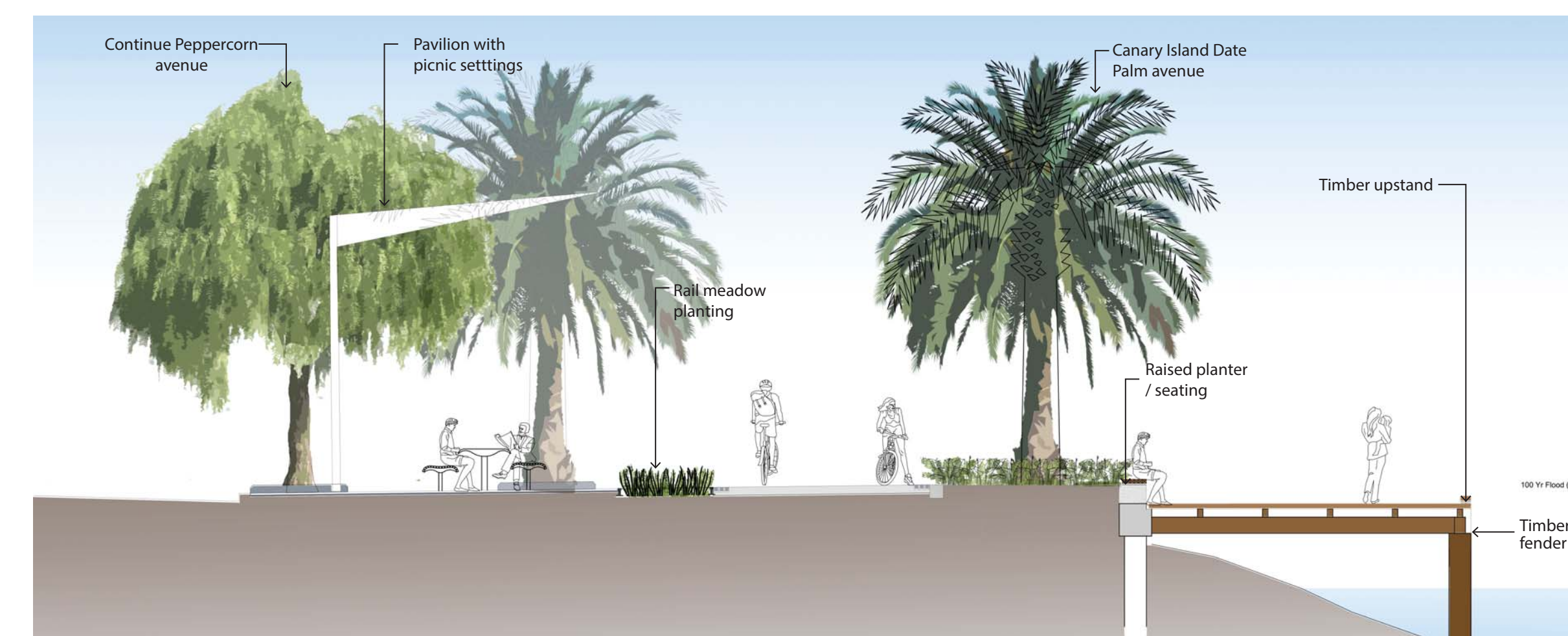
SECTION G-G
