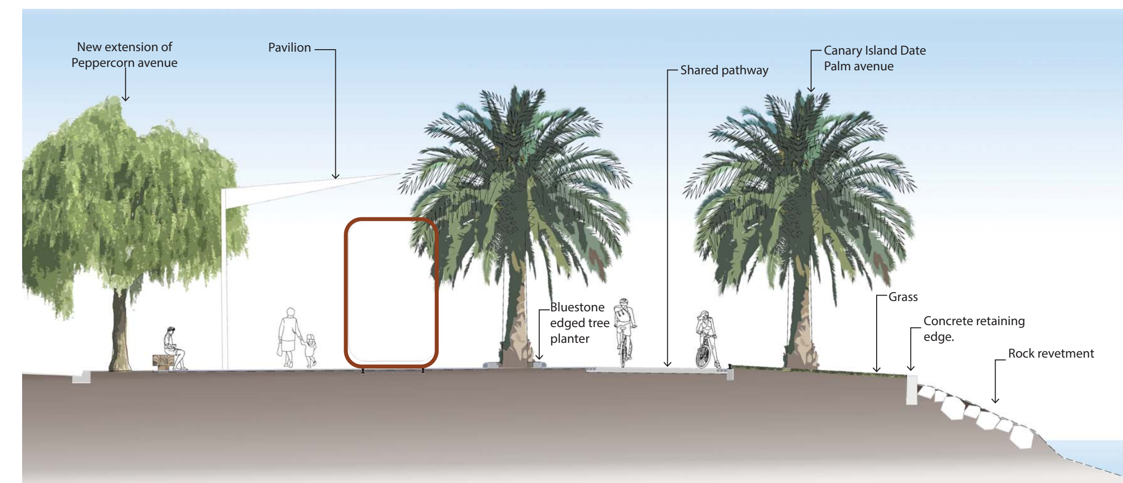
SECTION B-B
